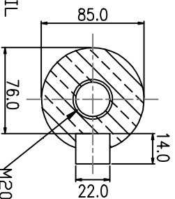
SHAFT DETAIL
