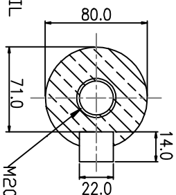
SHAFT DETAIL
