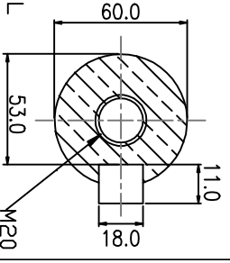
SHAFT DETAIL
