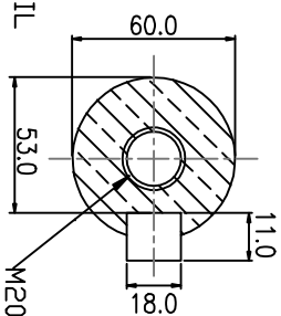
SHAFT DETAIL
