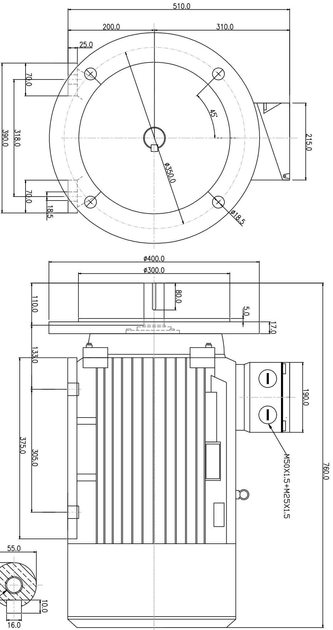
SHAFT DETAIL
