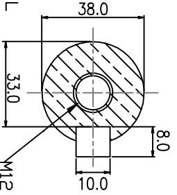
SHAFT DETAIL
