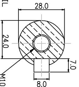
SHAFT DETAIL
